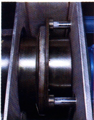
Air-activated choke for less maintenance, better control than spring-activated designs
